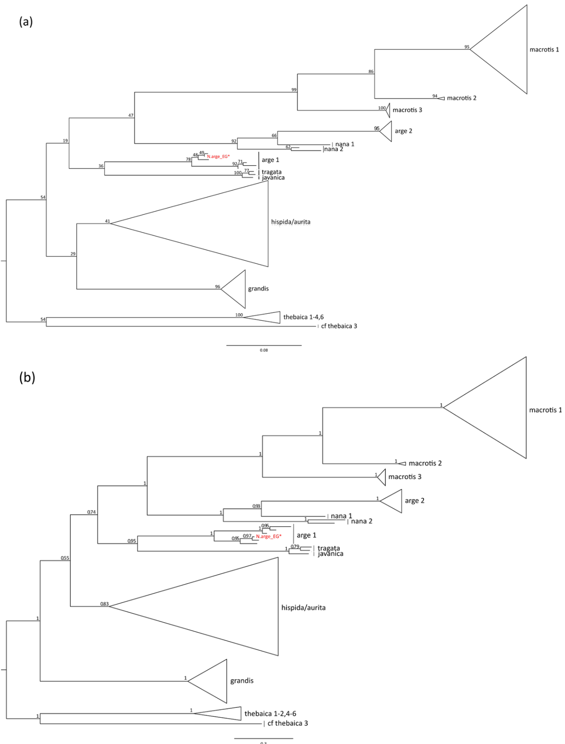
Fig. 1 - a) Maximum-likelihood and b) Bayesian phylogenetic trees based on partial cytochrome b DNA sequences. Values on nodes show Bootstrap values and Bayesian posterior probabilities. Piebald Nycteris arge captured in Equatorial Guinea (EG) is highlighted on red. See Demos et al (2019) for more information on samples used and Nycteris clades.
